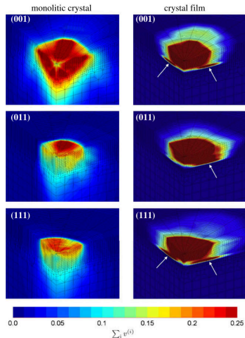
Spherical indentation of FCC copper crystal using crystal plasticity model in Zset
