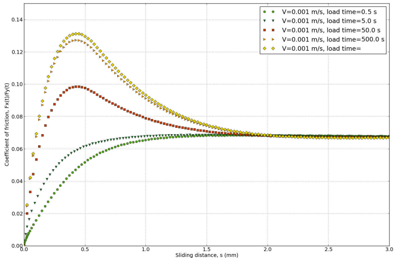
Effect of bringing-in-contact rate on frictional force evolution
