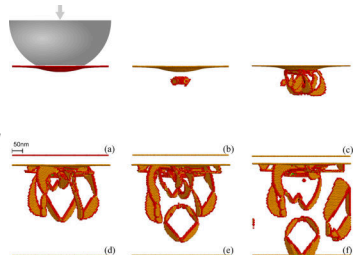
MD simulation of a spherical indentation on (111) FCC cube
