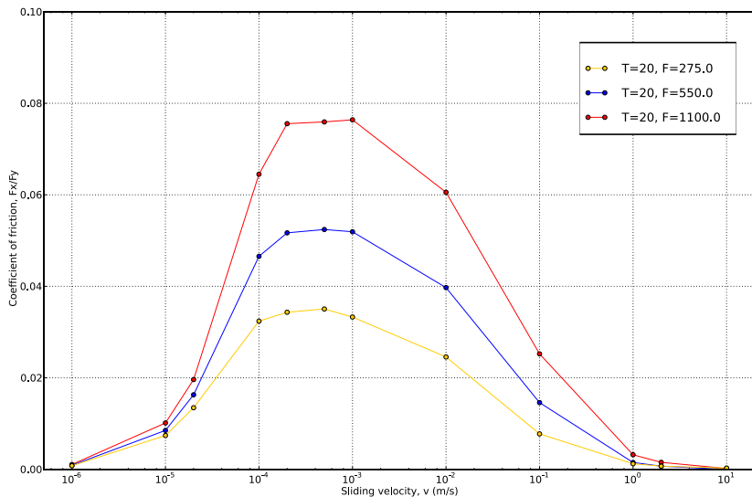
Frictional force at different slip velocity (effect of force)
